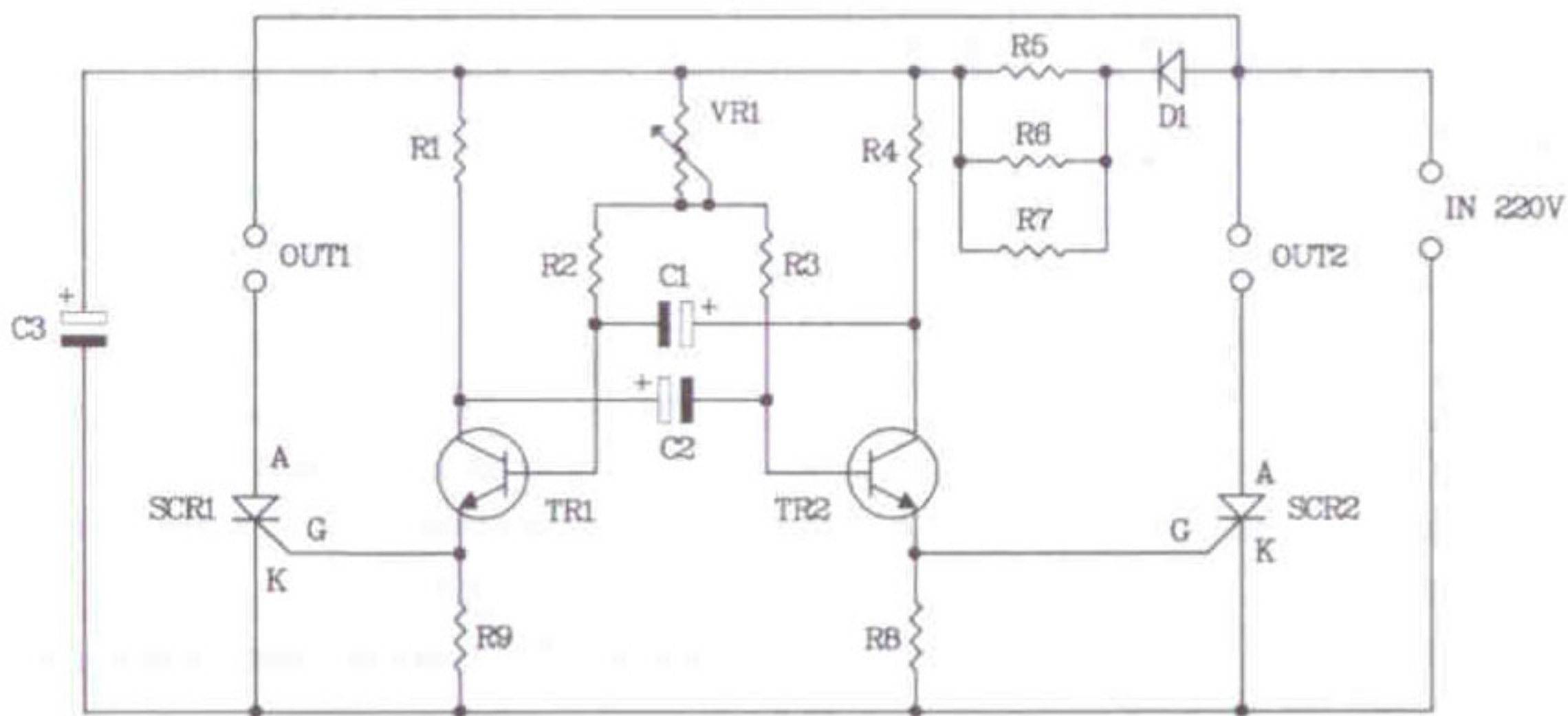
Figure 2. The AC flasher 2 CH. 1,400W. circuit
