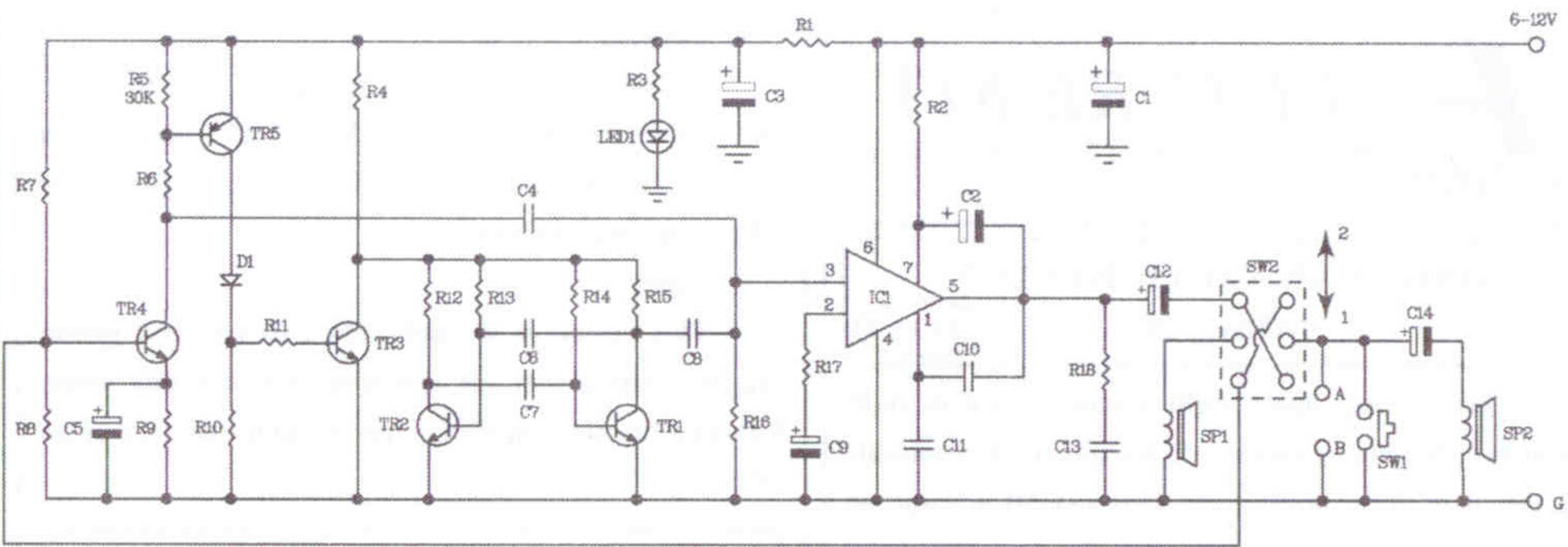
Figure 2. The dual station intercom&door bell circuit
