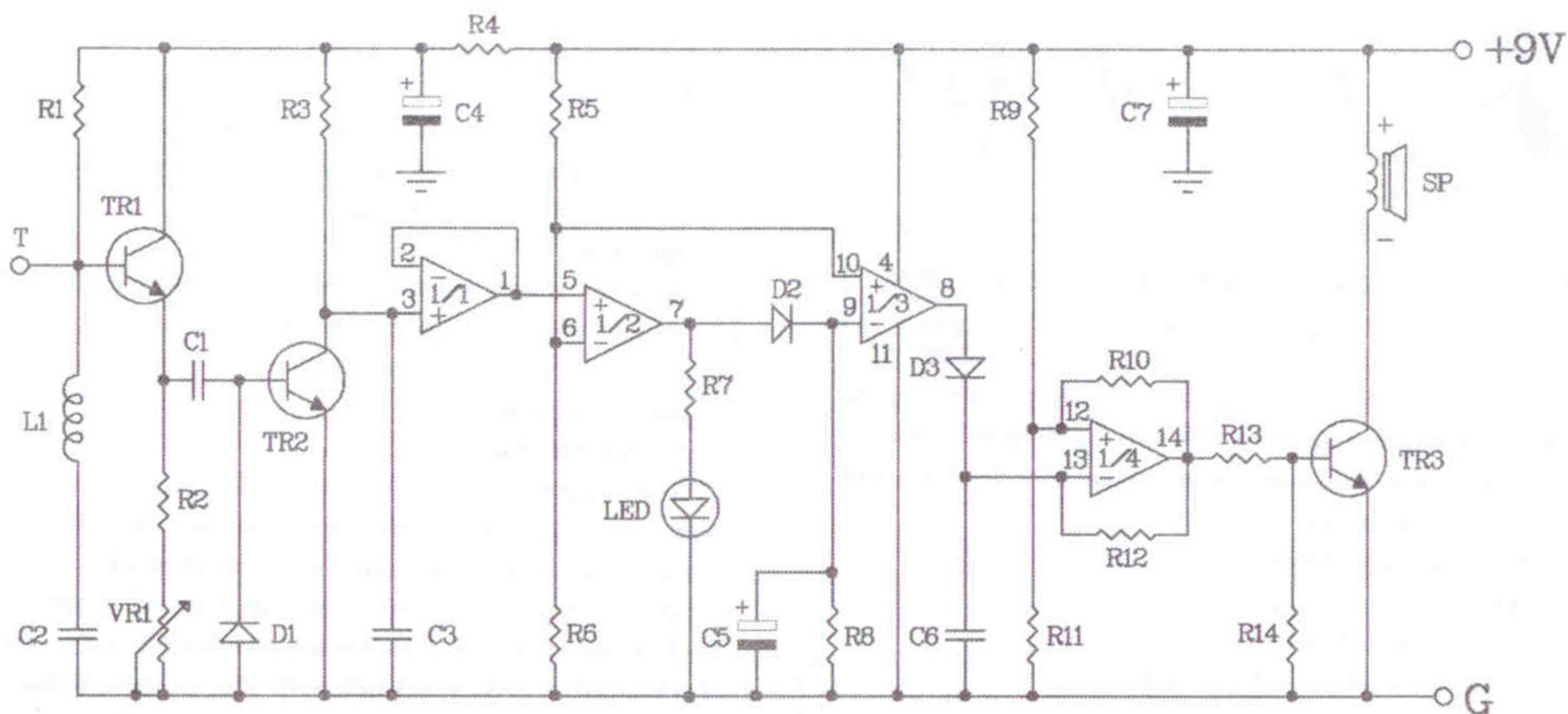
Figure 2. The door knob touch alarm circuit
