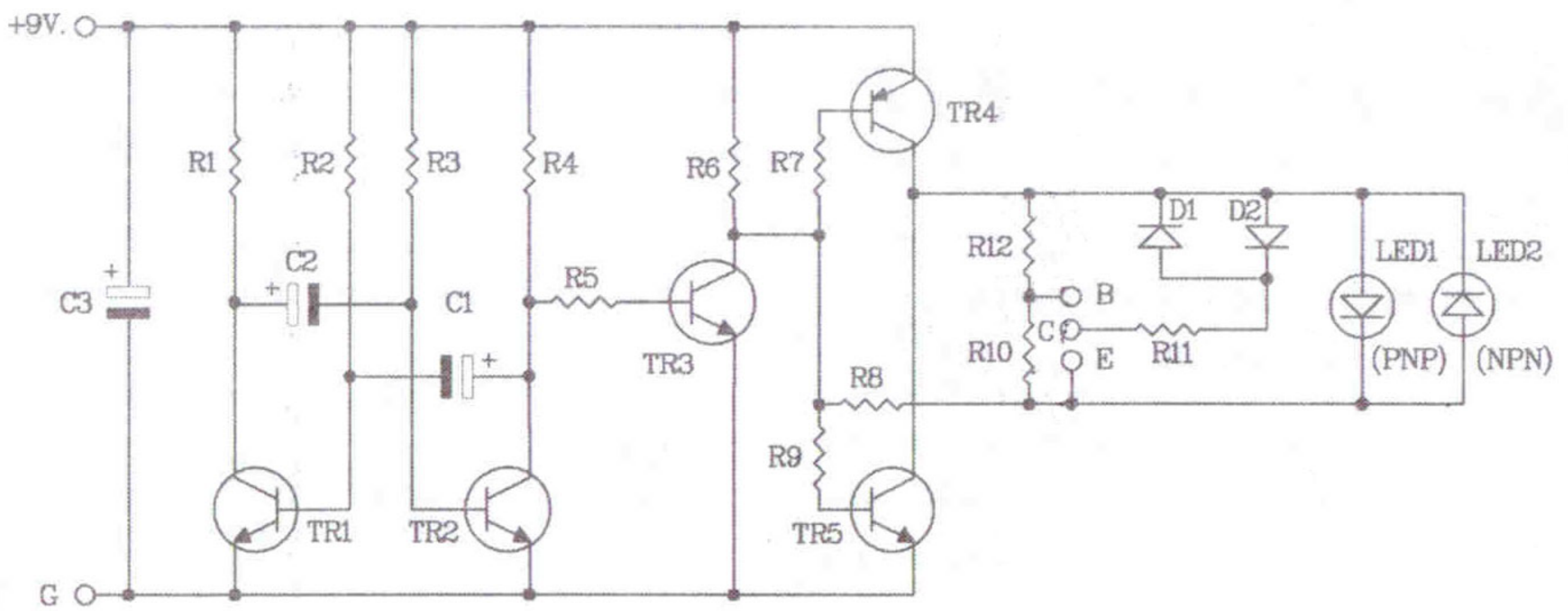
Figure 2. The in circuit TR checker circuit
