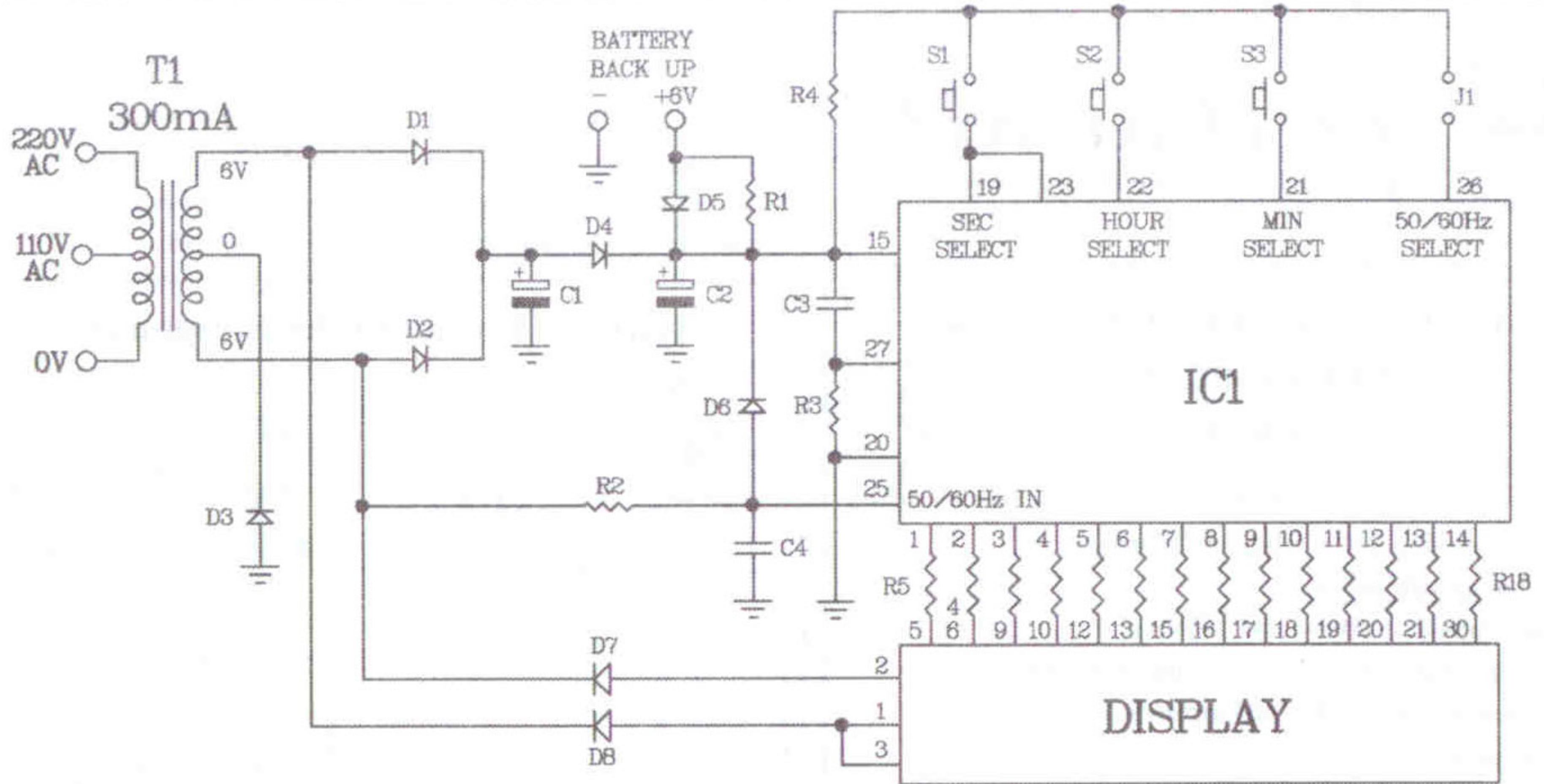
Figure 2. The digital clock (LED display) circuit
