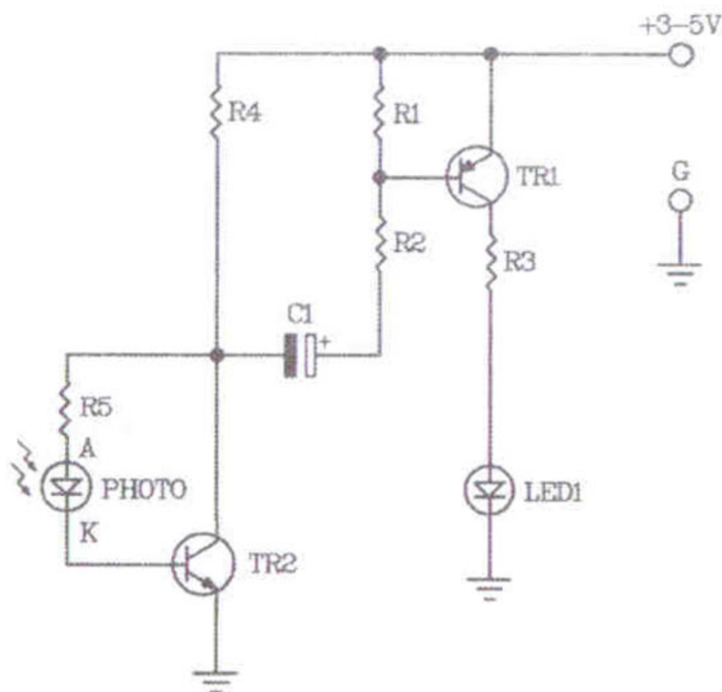
Figure 2. The infrared remote checker circuit
